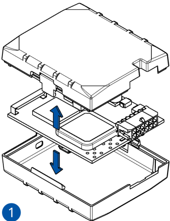
Figure 4 Covers removal
