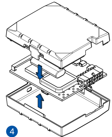
Figure 7 Cover removal
